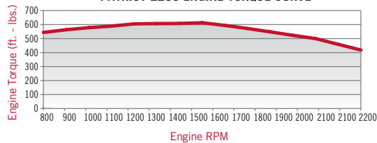
PATRIOT 2230 ENGINE TORQUE CURVE
