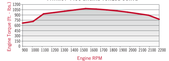
PATRIOT 4430 ENGINE TORQUE CURVE
