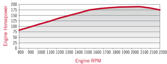
PATRIOT 2230 HORSEPOWER CURVE
