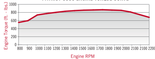
PATRIOT 3330 ENGINE TORQUE CURVE
