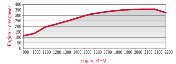
PATRIOT 4430 HORSEPOWER CURVE
