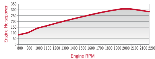
PATRIOT 3330 HORSEPOWER CURVE
